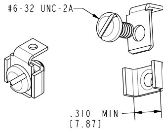
SCREW (AND CAGE) TERMINAL
